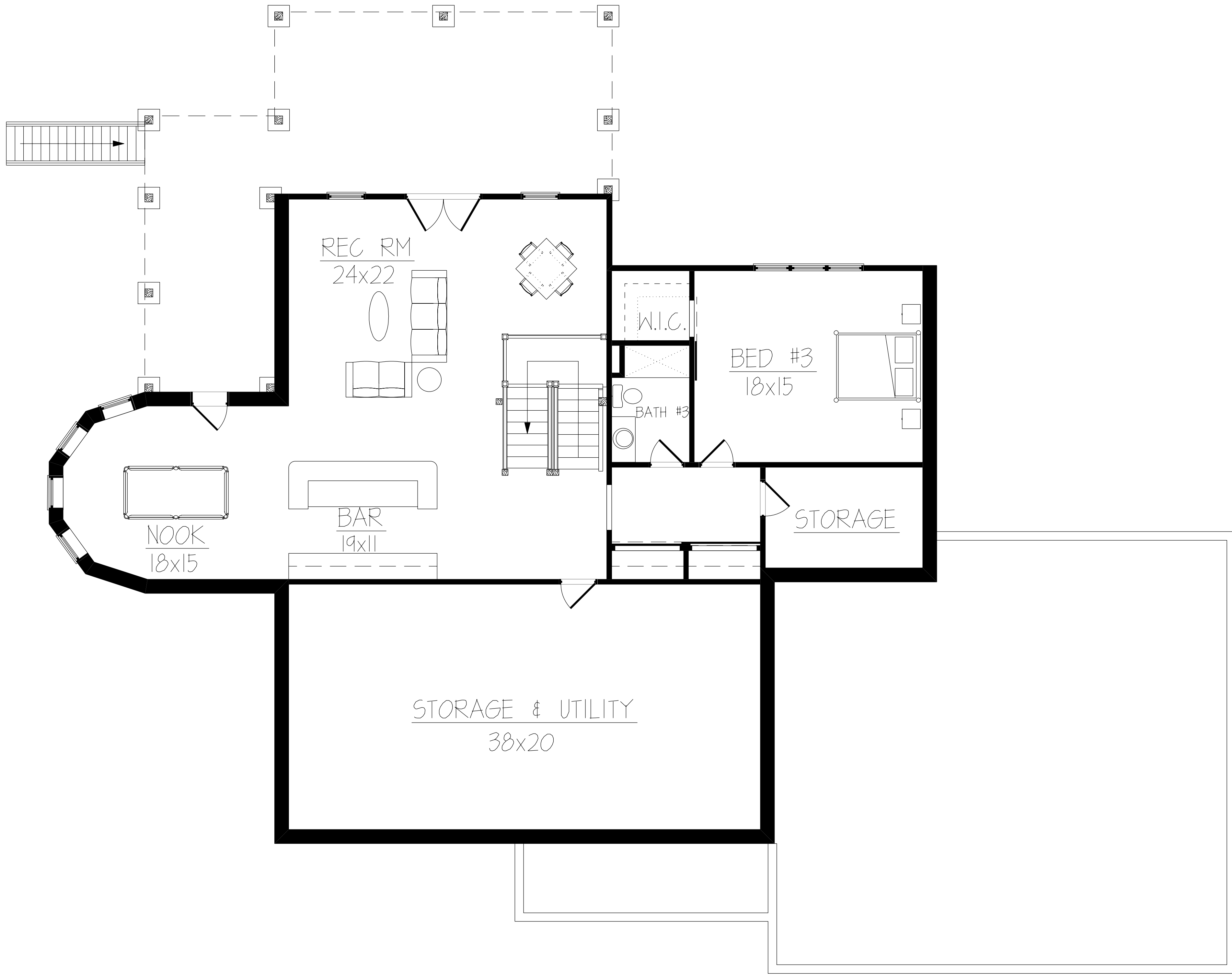
LOWER LEVEL FLOOR PLAN
