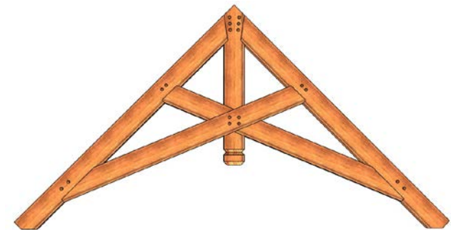
4X Scissor Truss
