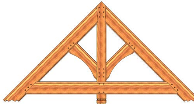
4X King Post Truss
