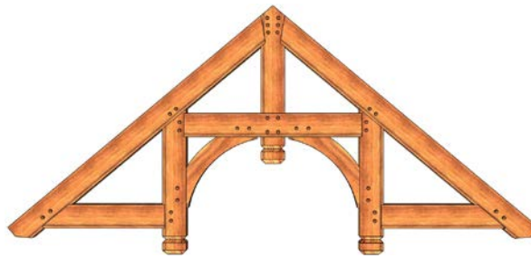
4X Hammer Beam Truss
